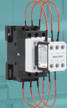
Capacitor Duty Contactor Ratings - 3 kVAr to 66 kVAr
